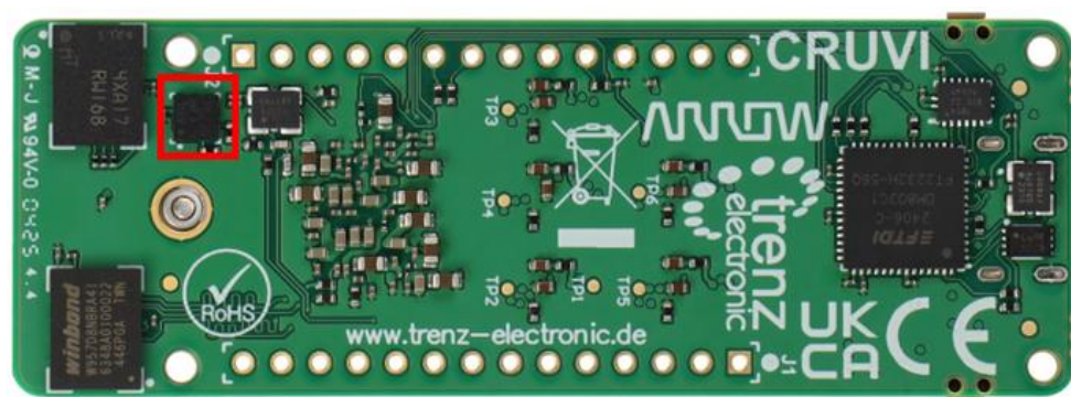
Figure 3-4 : Accelerometer location
